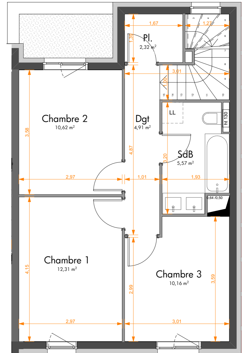
PLAN R+1
